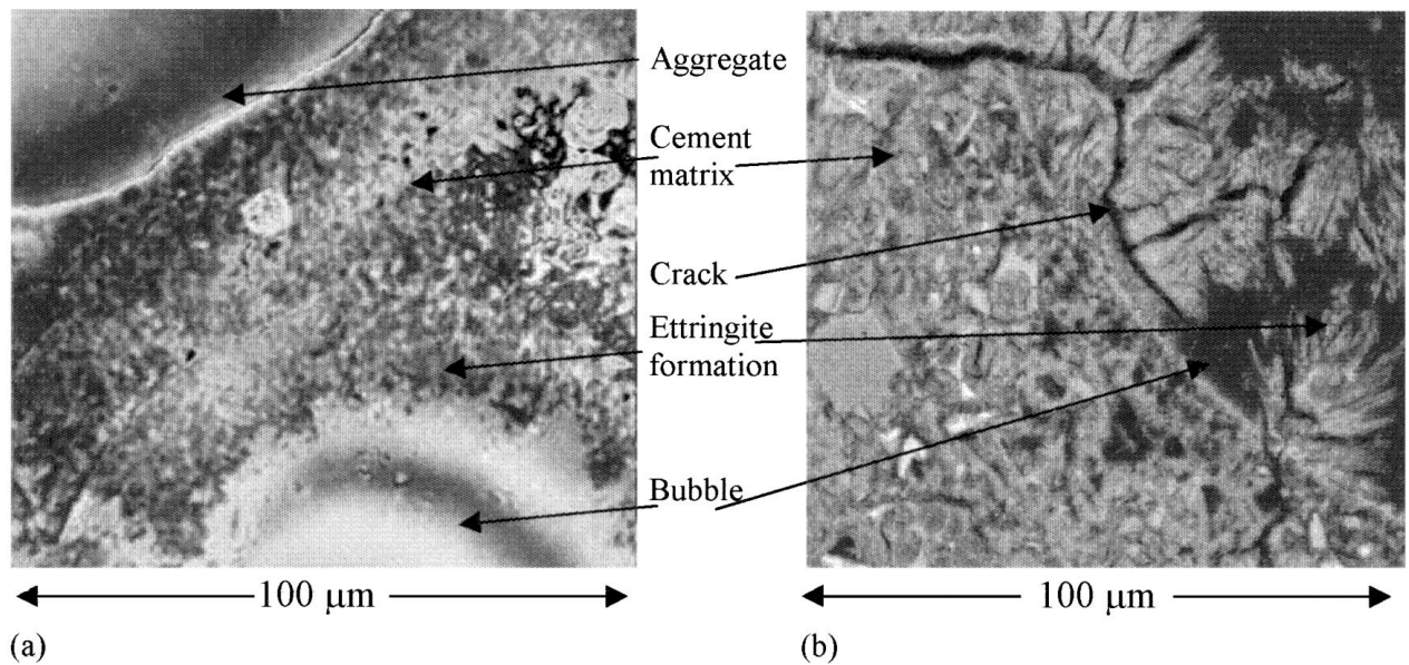
Figure 6 Acoustic C-scan (a) and SEM (b) images of the damaged concrete sample from a precasting plant. The image clearly shows a rim around the bubble. Elongated texture within the rim is due to crystals of ettringite. The acoustic image was made at 1 GHz. In SEM image, cracks have been formed due during the process of coating and putting the sample under vacuum.
