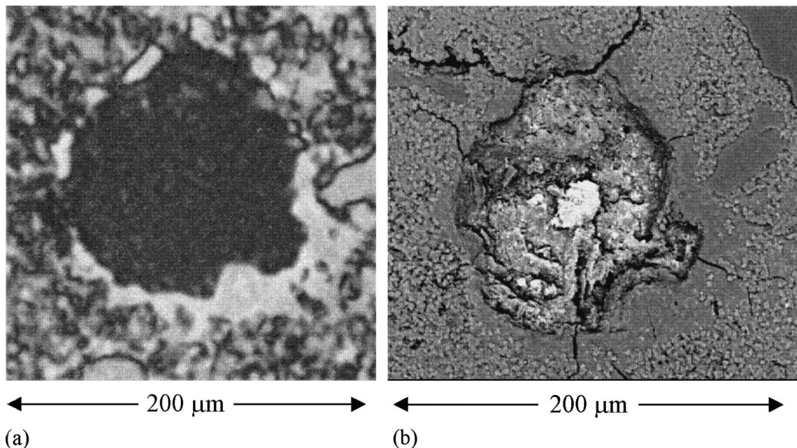
Figure 5 Bubble in cement mortar; (a) acoustical image made at 400 MHz; (b) SEM image.
