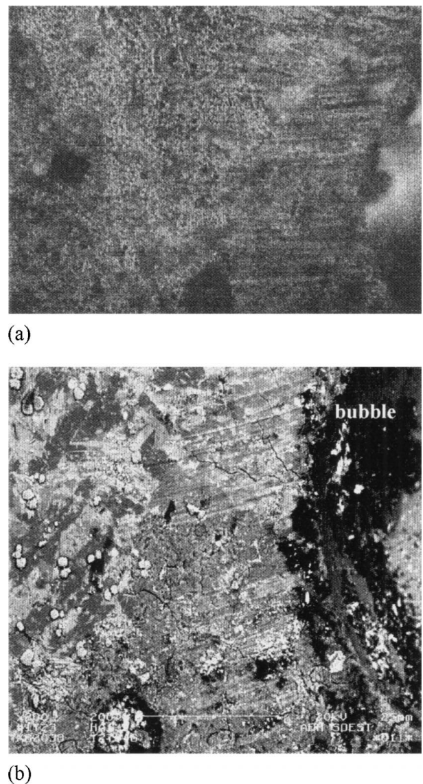
Figure 4 (a) reflected light optical, and (b) SEM images of of same area of the specimen shown in Fig. 3. The magnification of the optical image is 50 \times 1.25 .
