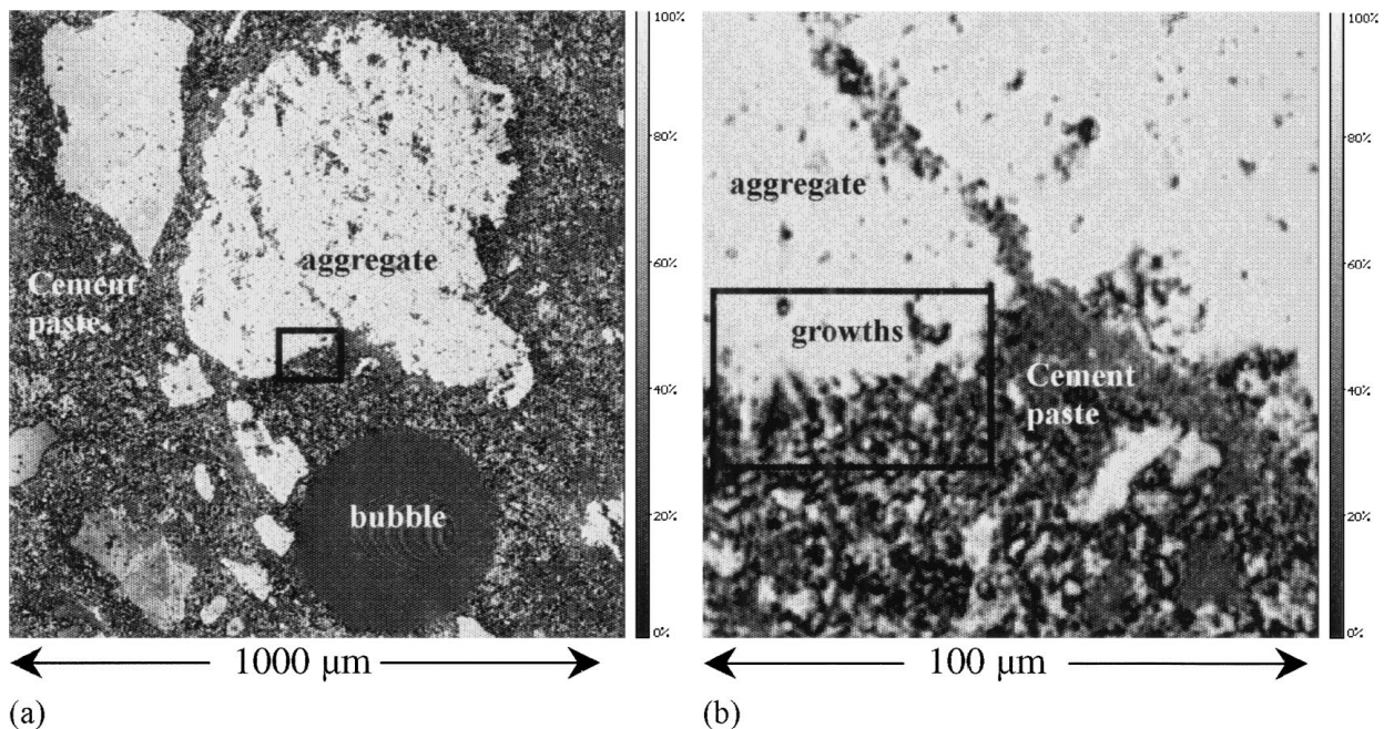
Figure 2 Acoustic images of a concrete mortar sample made with andesitic aggregate grains and with Portland cement paste. The acoustic image was made at 1 GHz, z = 0 . The box in (a) marks position of the high magnification acoustic image (b).
