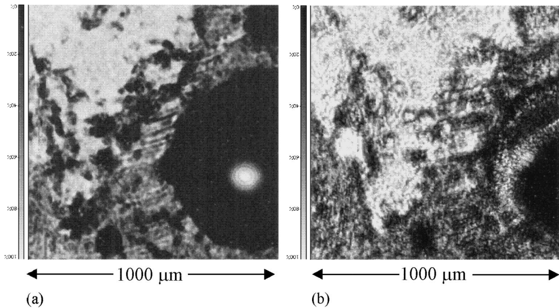
Figure 3 Acoustical micrographs of a concrete specimen made of andesitic aggregate grains in Portland cement paste with silica fume. (a): frequency 400 MHz; defocus Z = 0 \mu\text{m} . (b): frequency 200 MHz; defocus Z = -100 \mu\text{m} .
