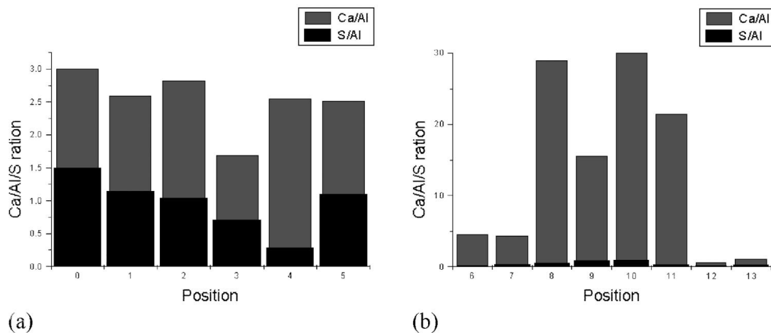
Figure 7 EDS analyses of the various components shown in Fig. 7a. Columns 1 to 5 contain data of positions in the reaction rim, columns 6 to 11 at increasing distance from the rim, data in column 12 and 13 was collected from aggregate grains, and column 0 shows EDS analyses of a standard ettringite sample (Ca : Al : S = 3 : 1 : 1.5).
